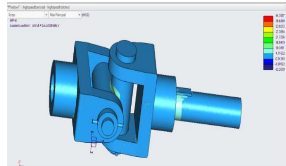
Principle stress of High speed tool steel
