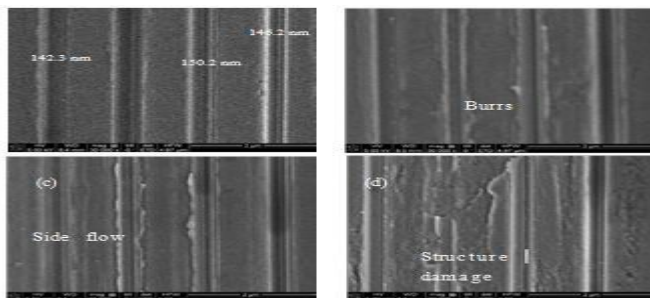
Fig 4.3 SEM images of Nano-grooves machined using different depth of cut. (a) 100 nm; (b) 200 nm; (c) 300 nm; (d) 400 nm. (Spindle speed = 12 rpm, feed rate = 9 μm/re).
