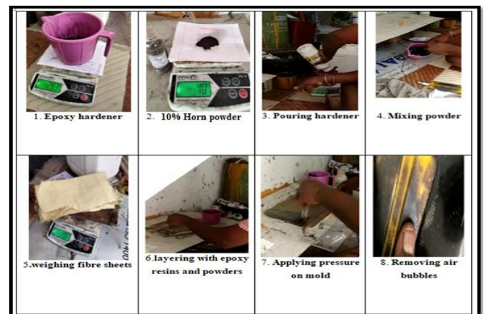
Figure 19 Complete sequential process for fabrication
