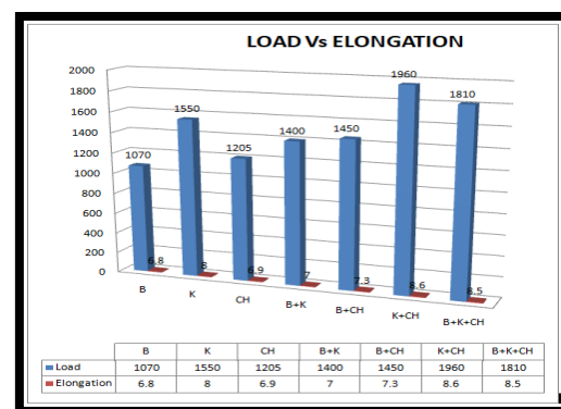
Graph 2 Flexuraltestresultgraph
