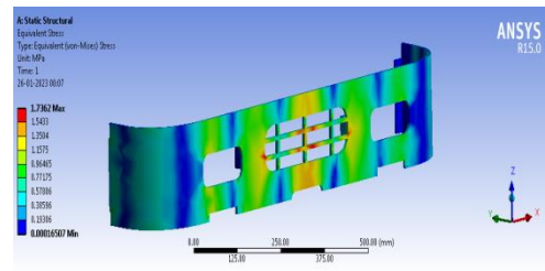
Figure 35 Von-mises stress of ALB390 Material
