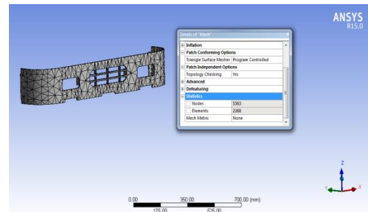
Figure 30 MESHING: NODES: 5363 ELEMENTS: 2268
