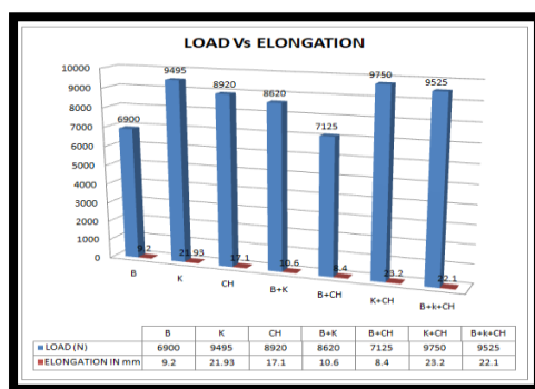
Graph 1 tensiletestresultgraph
