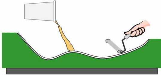
Fig: handmade lay-up process
