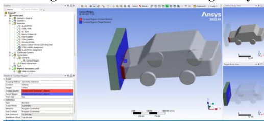
Figure7: Contact region
