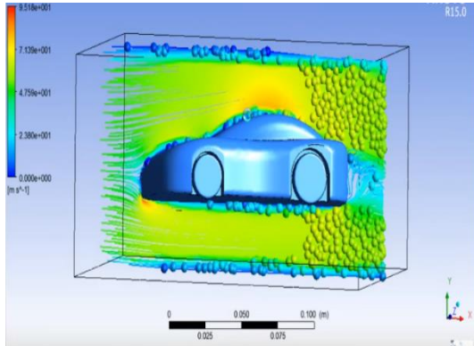
Figure31: maximum - velocity of the racing car
