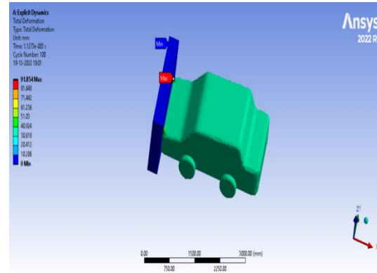
Figure 19: Total deformation
