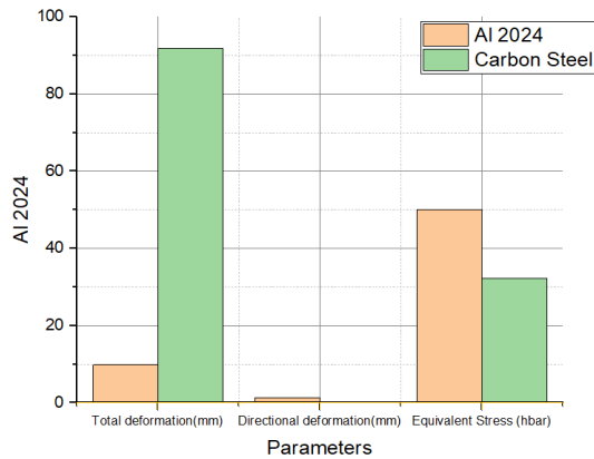
Graph 1: Explicit Dynamic Analysis of Hybrid Drive Racing Car Using different materials
