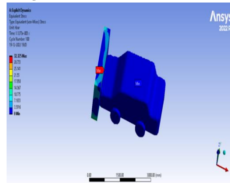
Figure 21: Equivalent stress Table: Explicit Dynamic Analysis of Hybrid Drive Racing Car Using different materials Maximum deformations
