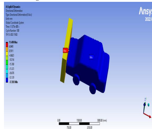
Figure 20: Directional deformation
