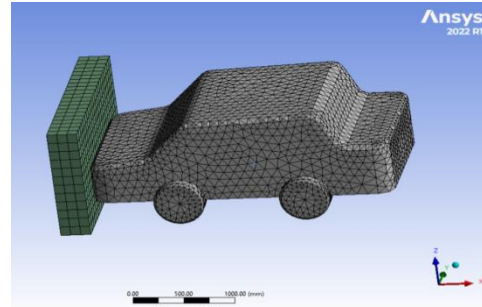
Figure 8: Meshed model
