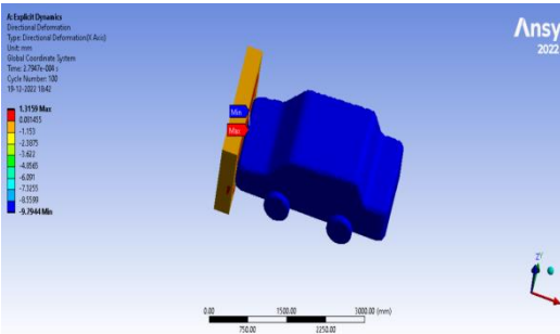
Figure 16: Directional deformation
