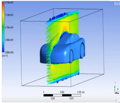
Figure 30: racing car velocity of steam line
