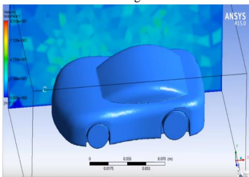
Figure 26: Complete Distribution of Velocity
