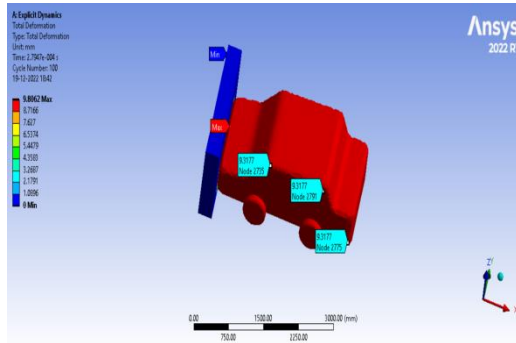
Figure 15: Total deformation
