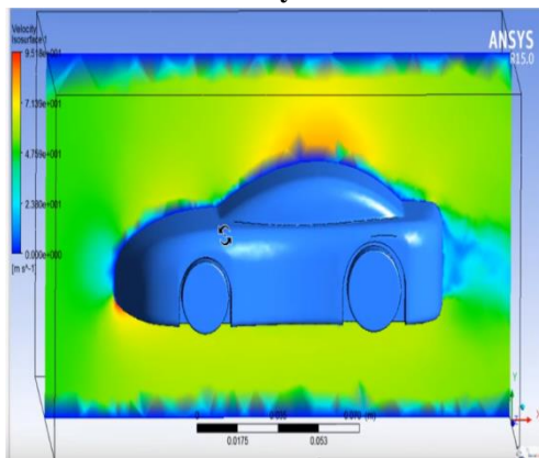
Figure 25: Distribution Velocity of The Racing Car
