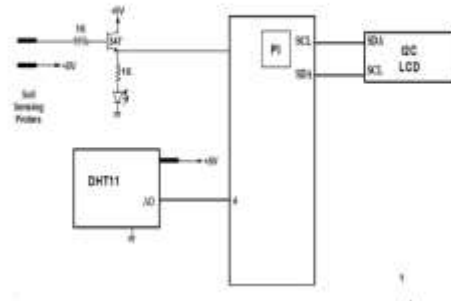
Fig 8. Schematic Diagram
