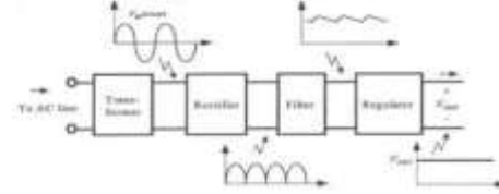
Figure 5: Block Diagram of Power Supply
