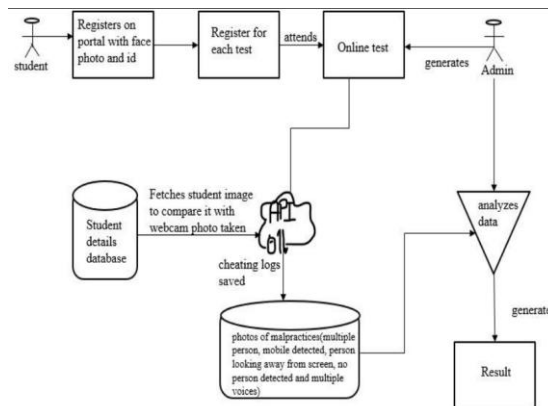
Figure 1: System Methodology
