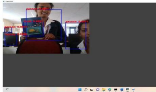
Figure 7: Objects Detection
